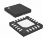
PIC16LF1509T-I/GZ Microchip Technology IC MCU 8BIT 14KB FLASH 20UQFN
