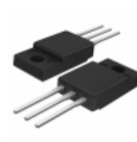
BTA410X-800ET,127 WeEn Semiconductors TRIAC SENS GATE 800V 10A TO220F
