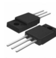
BTA410X-800CT,127 WeEn Semiconductors TRIAC 800V 10A TO220F
