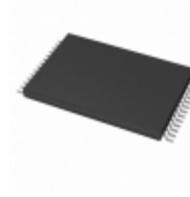
AT27BV256-70TU Microchip Technology IC OTP 256KBIT 70NS 28TSOP
