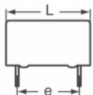
B32796G8106J EPCOS (TDK) CAP FILM 10UF 5% 875VDC RADIAL
