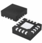
MCP4241-104E/ML Microchip Technology IC POT DGTL DUAL 100K SPI 16QFN
