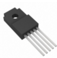
BAJ2CC0WT Rohm Semiconductor IC REG LDO 12V 1A TO220FP-5
