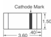
DL5259B-TP Micro Commercial Co DIODE ZENER 39V 500MW MINIMELF
