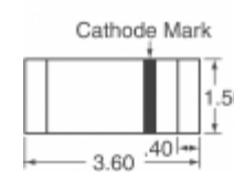
DL5258B-TP Micro Commercial Co DIODE ZENER 36V 500MW MINIMELF
