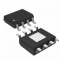
MIC37301-2.5YME Microchip Technology IC REG LDO 2.5V 3A 8SOIC
