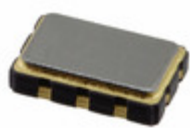
LDF620001 Diodes Incorporated OSCILLATOR XO 156.25MHZ LVDS SMD
