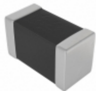
EMK316BJ475ML-T Taiyo Yuden CAP CER 4.7UF 16V X5R 1206
