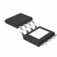
BD00FC0WFEJ-E2 Rohm Semiconductor IC REG LDO ADJ 1A 8HTSOPJ
