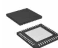
DSPIC30F4012T-20E/ML Microchip Technology IC MCU 16BIT 48KB FLASH 44QFN
