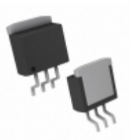
MCP1826ST-1202E/EB Microchip Technology IC REG LDO 1.2V 1A 3DDPAK
