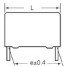
B32924C3275K000 EPCOS CAP FILM 2.7UF 10% 305VAC RADIAL
