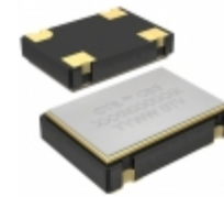
CB3LV-3C-2M5000 CTS-Frequency Controls OSC XO 2.5MHZ HCMOS TTL SMD
