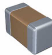
C0603C270J4HAC7867 KEMET CAP CER 0603 27PF 16V ULTRA STAB
