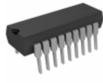
PIC16C620-04I/P Microchip Technology IC MCU 8BIT 896B OTP 18DIP
