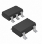
MIC5259-2.5YD5-TR Microchip Technology IC REG LDO 2.5V 0.3A TSOT23-5
