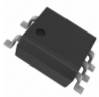
ACPL-M72T-560E Broadcom Limited OPTOISO 4KV PUSH PULL 5SO
