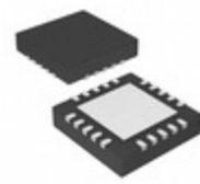
MCP4451T-502E/ML Microchip Technology IC DGTL POT 257POS 5K 20QFN
