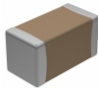
CDR32BP3R3BCZRAT Vishay Vitramon CAP CER 3.3PF 100V BP 1206
