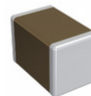
GRM21B5C1H223FA01L Murata Electronics CAP CER 0.022UF 50V COG/NP0 0805
