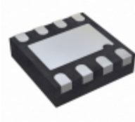
ADA4610-2ACPZ-R7 Analog Devices Inc. IC OPAMP JFET 16.3MHZ RRO 8LFCSP
