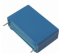
B32676G3206K000 EPCOS CAP FILM 20UF 10% 300VDC RADIAL
