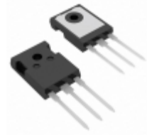
IXSH40N60A IXYS IGBT 600V 75A 300W TO247AD
