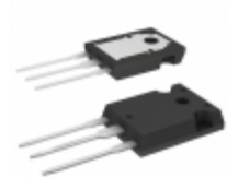
TIP34C STMicroelectronics TRANS PNP 100V 10A TO-247
