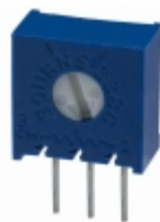
3386C-1-503LF Bourns, Inc. TRIMMER 50K OHM 0.5W PC PIN SIDE
