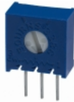
3386C-1-502LF Bourns, Inc. TRIMMER 5K OHM 0.5W PC PIN SIDE
