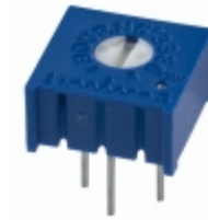
3386F-1-100LF Bourns, Inc. TRIMMER 10 OHM 0.5W PC PIN TOP
