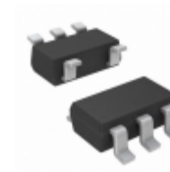
TC2055-1.8VCTTR Microchip Technology IC REG LDO 1.8V 0.1A SOT23-5
