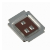
IRF6648TR1PBF Infineon Technologies MOSFET N-CH 60V 86A DIRECTFET
