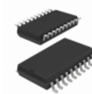
TLE4262GNTMA1 Infineon Technologies IC REG LDO 5V 0.15A 20DSO
