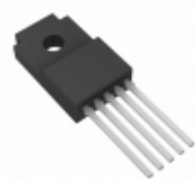
BA33DD0WT Rohm Semiconductor IC REG LDO 3.3V 2A TO220FP
