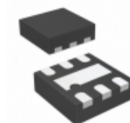
MIC94345-SYMT-T5 Microchip Technology IC REG LDO 3.3V 0.5A 6TDFN
