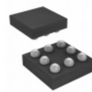
AS13986-1833-T ams IC REG LDO 1.8V/3.3V 0.15A 8WLP
