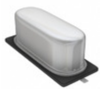
ABLS-8.000MHZ-B4-T Abracon LLC CRYSTAL 8.000MHZ 18PF SMD
