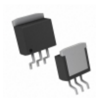
MIC39150-1.8BU TR Microchip Technology IC REG LDO 1.8V 1.5A TO263-3
