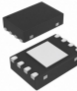
11LC161T-I/MNY Microchip Technology IC EEPROM 16KBIT 100KHZ 8TDFN
