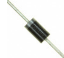
MUR490E ON Semiconductor DIODE GEN PURP 900V 4A DO201AD
