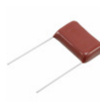
ECQ-E2225KF Panasonic Electronic Components CAP FILM 2.2UF 10% 250VDC RADIAL
