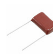
ECQ-E2225JFW Panasonic Electronic Components CAP FILM 2.2UF 5% 250VDC RADIAL
