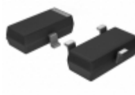
BAS 40 B5003 Infineon Technologies DIODE SCHOTTKY 40V 120MA SOT23-3
