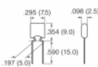
B37984M5824K054 EPCOS (TDK) CAP CER 0.82UF 50V X7R RADIAL
