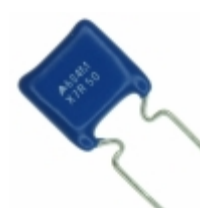
B37984M5684M051 EPCOS (TDK) CAP CER 0.68UF 50V X7R RADIAL
