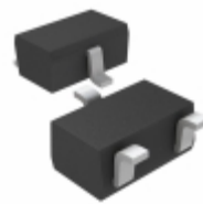
UMZ5.1NT106 Rohm Semiconductor DIODE ZENER ARRAY 5.1V UMD3
