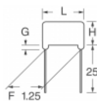
ECQ-P4223JU Panasonic Electronic Components CAP FILM 0.022UF 5% 400VDC RAD
