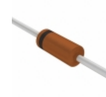
BZX55B3V6 A0G TSC (Taiwan Semiconductor) DIODE ZENER 3.6V 500MW DO35
