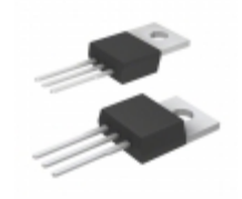
IXTP27N20T IXYS MOSFET N-CH 200V 27A TO-220
