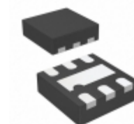
MIC94345-4YMT-TR Microchip Technology IC REG LDO 1.2V 0.5A 6TDFN
