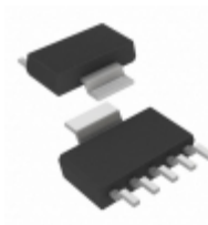
MCP1826T-1202E/DC Microchip Technology IC REG LDO 1.2V 1A SOT223-5
