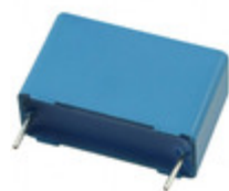
B32523Q6224J000 EPCOS CAP FILM 0.22UF 5% 400VDC RADIAL
