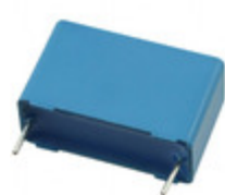
B32523Q6155K000 EPCOS CAP FILM 1.5UF 10% 400VDC RADIAL
