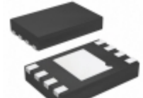
BU7262NUX-TR Rohm Semiconductor IC OPAMP GP 2MHZ RRO 8VSON
