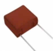
ECW-F2185JA Panasonic Electronic Components CAP FILM 1.8UF 5% 250VDC RADIAL
