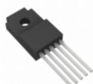
BA70BC0WT Rohm Semiconductor IC REG LDO 7V 1A TO220FP-5
